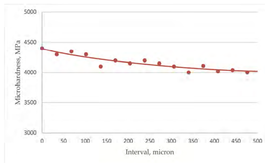
Figure 8. Depth distribution of microhardness of a nitrided ball head after 12 years of implantation in a human body (each experimental point is an average value based on the results of 5 measurements on one head).
