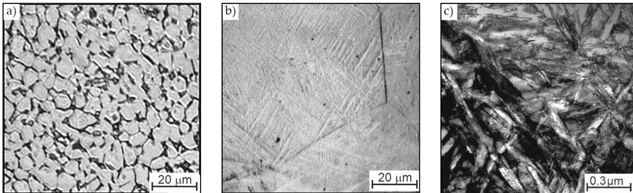
Figure 1. The structure of a ball heads in (a) the annealed state and after (b) hydrogenating annealing or (c) vacuum annealing.
