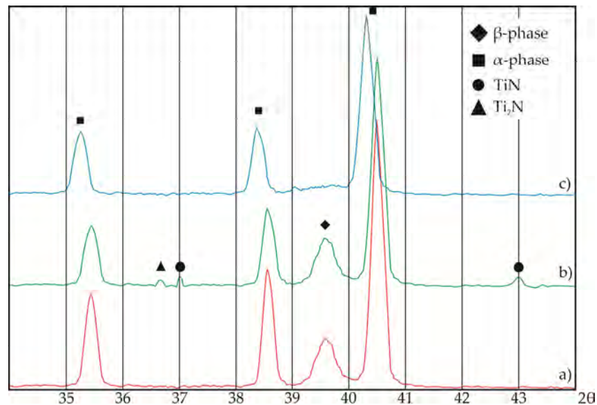
Figure 4. The X-ray diffraction of the ball heads (a) in the annealed state and after (b) THT and nitriding or (c) 12 years of implantation in a human body.
