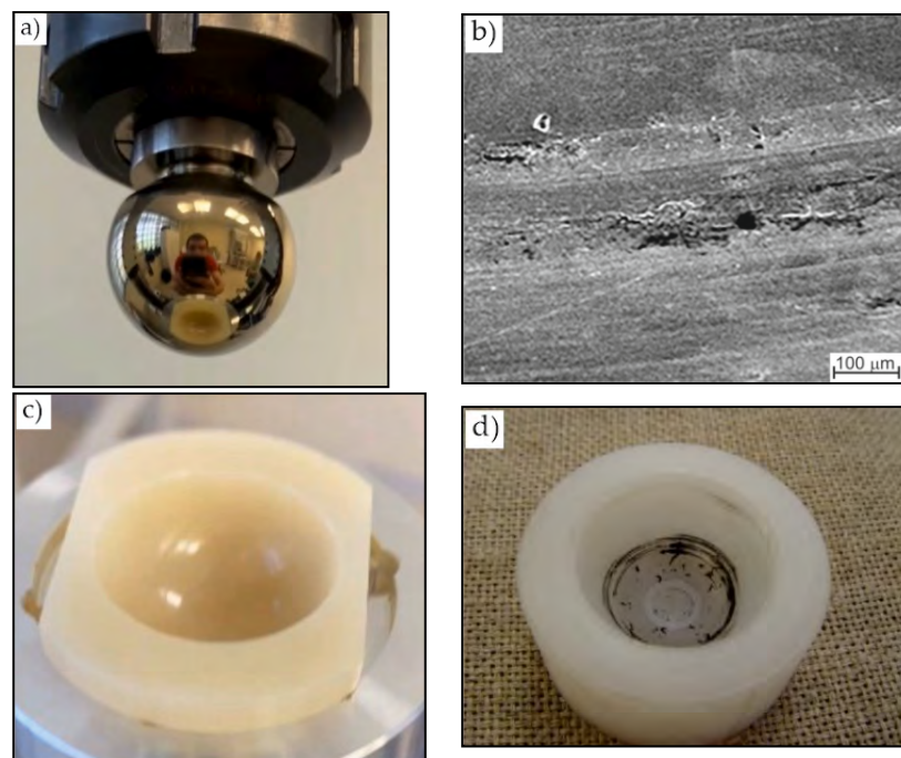
Figure 6. The appearance of (a,b) ball heads and (c,d) UHMWPE inserts with (a,c) modified and (b,d) unmodified surface after wear tests.
