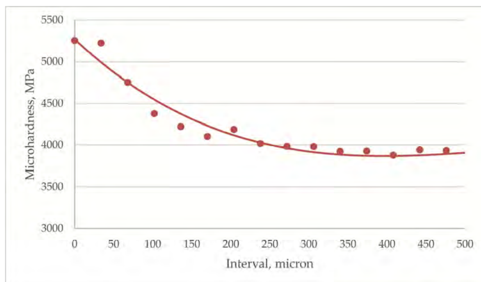
Figure 2. Depth distribution of microhardness of nitrided ball heads made of Ti-6Al-4V alloy (each experimental point is an average value based on the results of three measurements on five heads).
