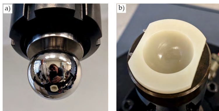
Figure 9. The appearance of (a) the removed ball head and (b) the UHMWPE inserts after wear testing.
