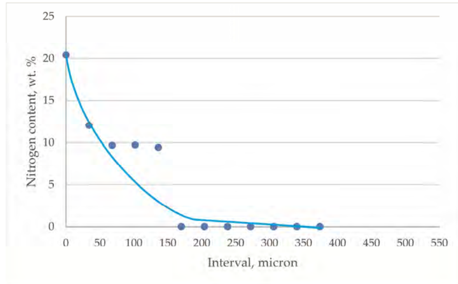
Figure 3. Depth distribution of nitrogen content of nitrided ball heads made of Ti-6Al-4V alloy (each experimental point is the average value of the results of five measurements on one head).
