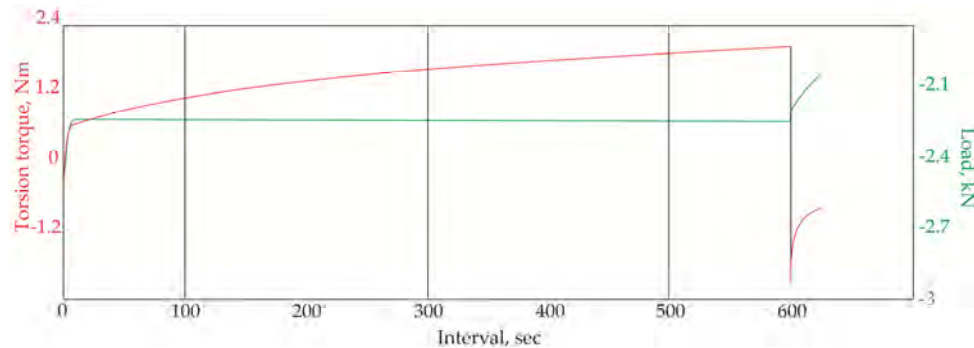
Figure 5. The torque and load during testing of the friction pair Ti–6Al–4V alloy ball head with modified surface—UHMWPE insert.
