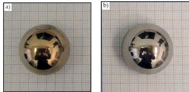
Figure 7. The appearance of the ball heads after (a) nitriding and (b) removal from a human body after 12 years of implantation.
